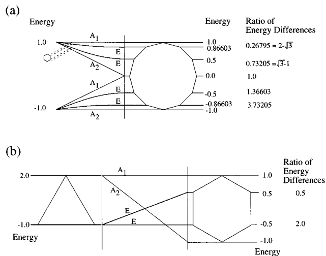
FIG. 7. Superfine structure of the subclusters D_{3d}-C_{3v} symmetry breaking. (a) 12-fold clusters found near C_3 axes. (b) Sixfold clusters found near C_5 axes.
