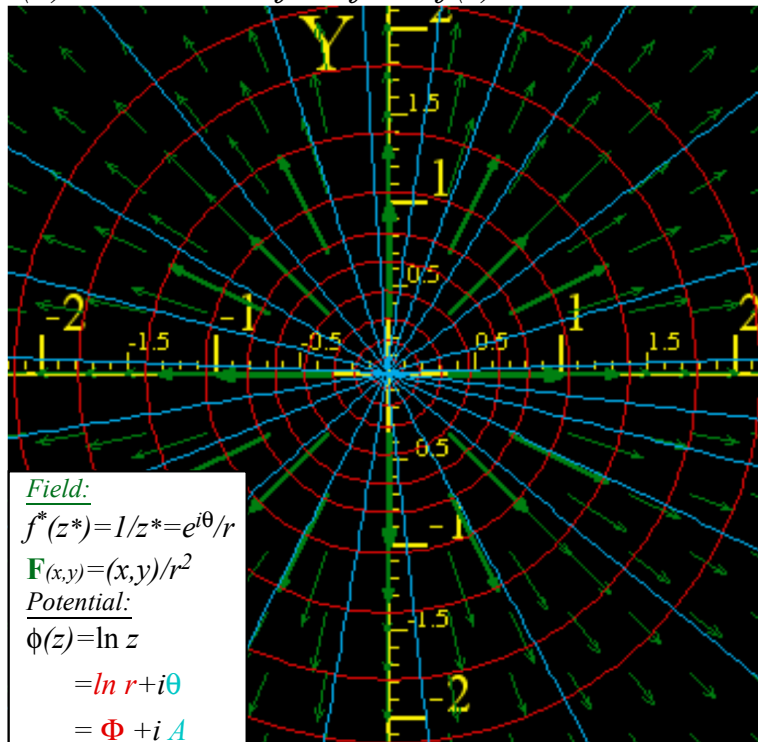
(a) Unit Z-line-flux field f(z)=1/z
