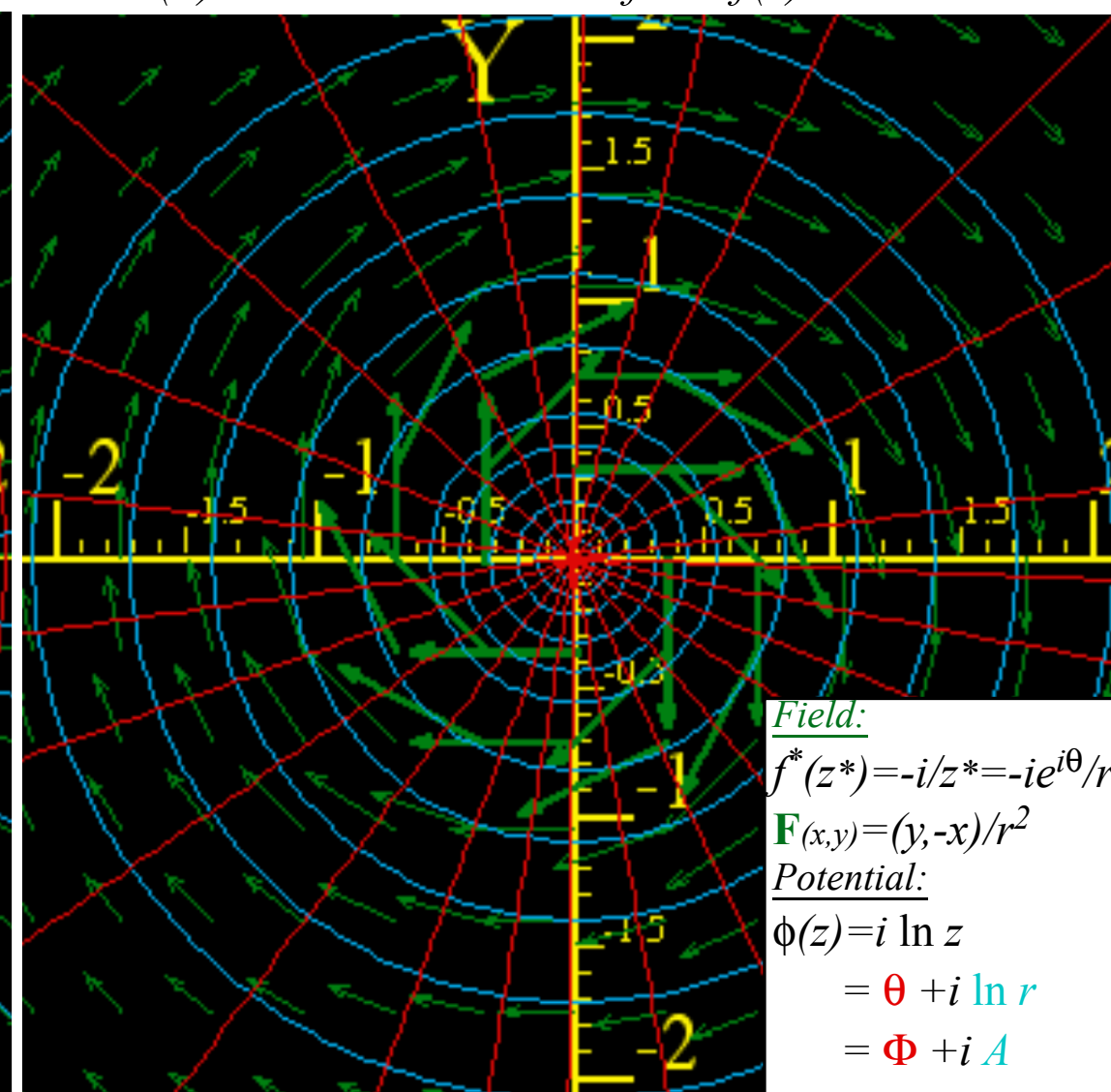
(b) Unit Z-line-vortex field f(z)=i/z
